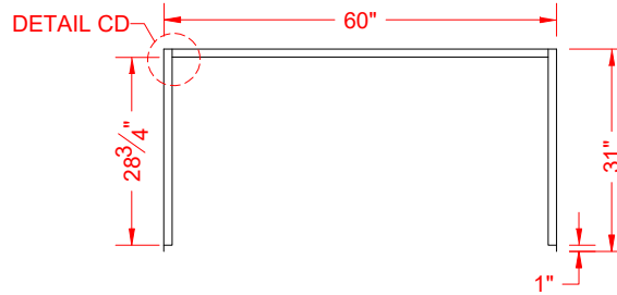
TOP VIEW - SCALE \frac{3}{8}'' = 1'-0''
