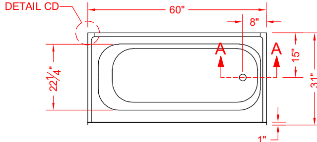
TOP VIEW - SCALE \frac{3}{8}'' = 1'-0''
